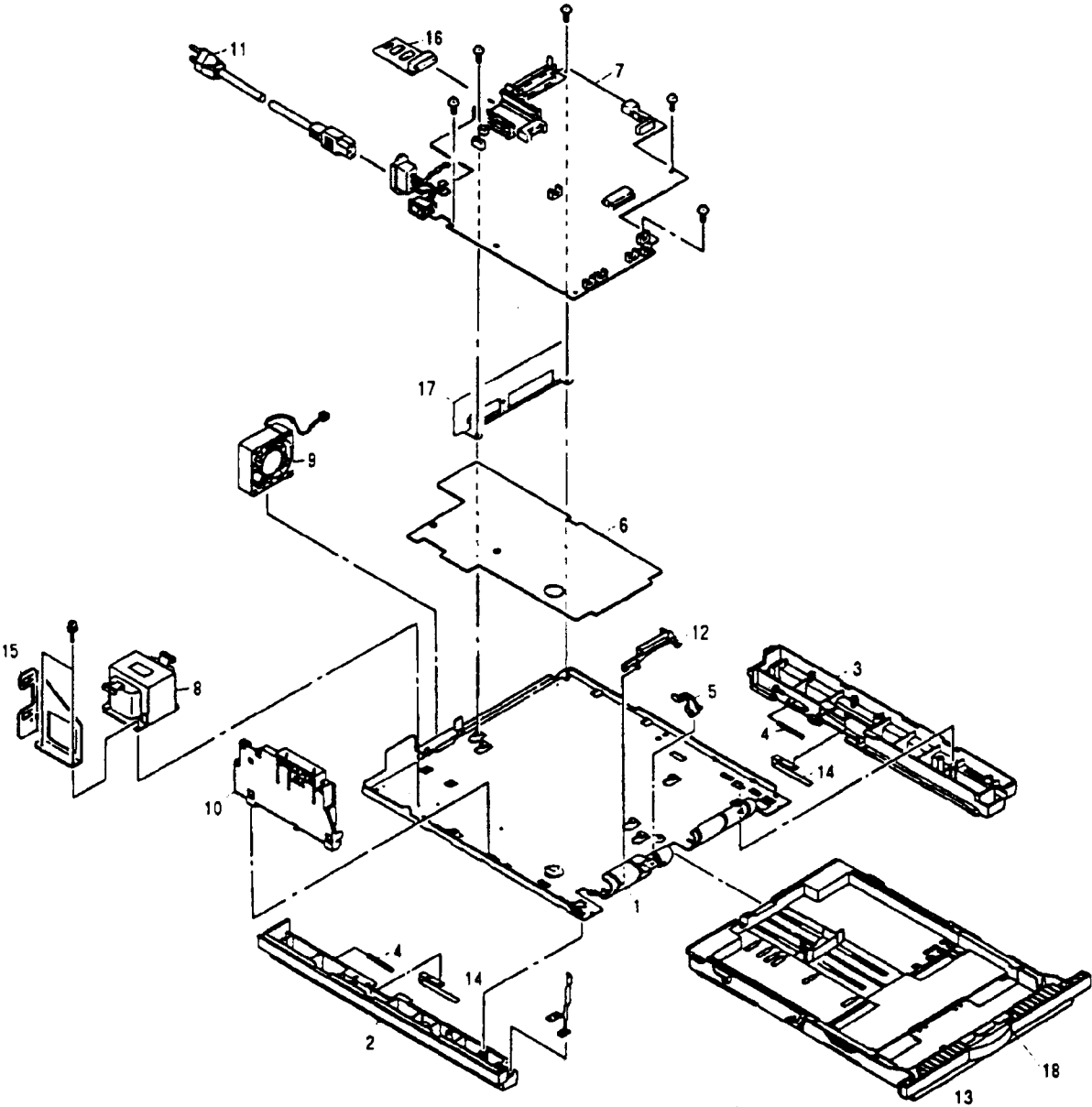
Figure 8-3 Base unit
