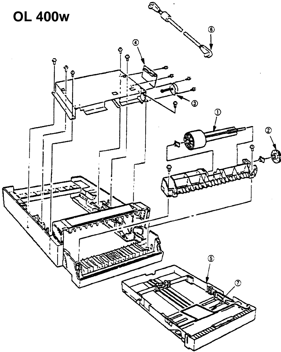
Figure 6-1 High Capacity Second Paper Feeder
