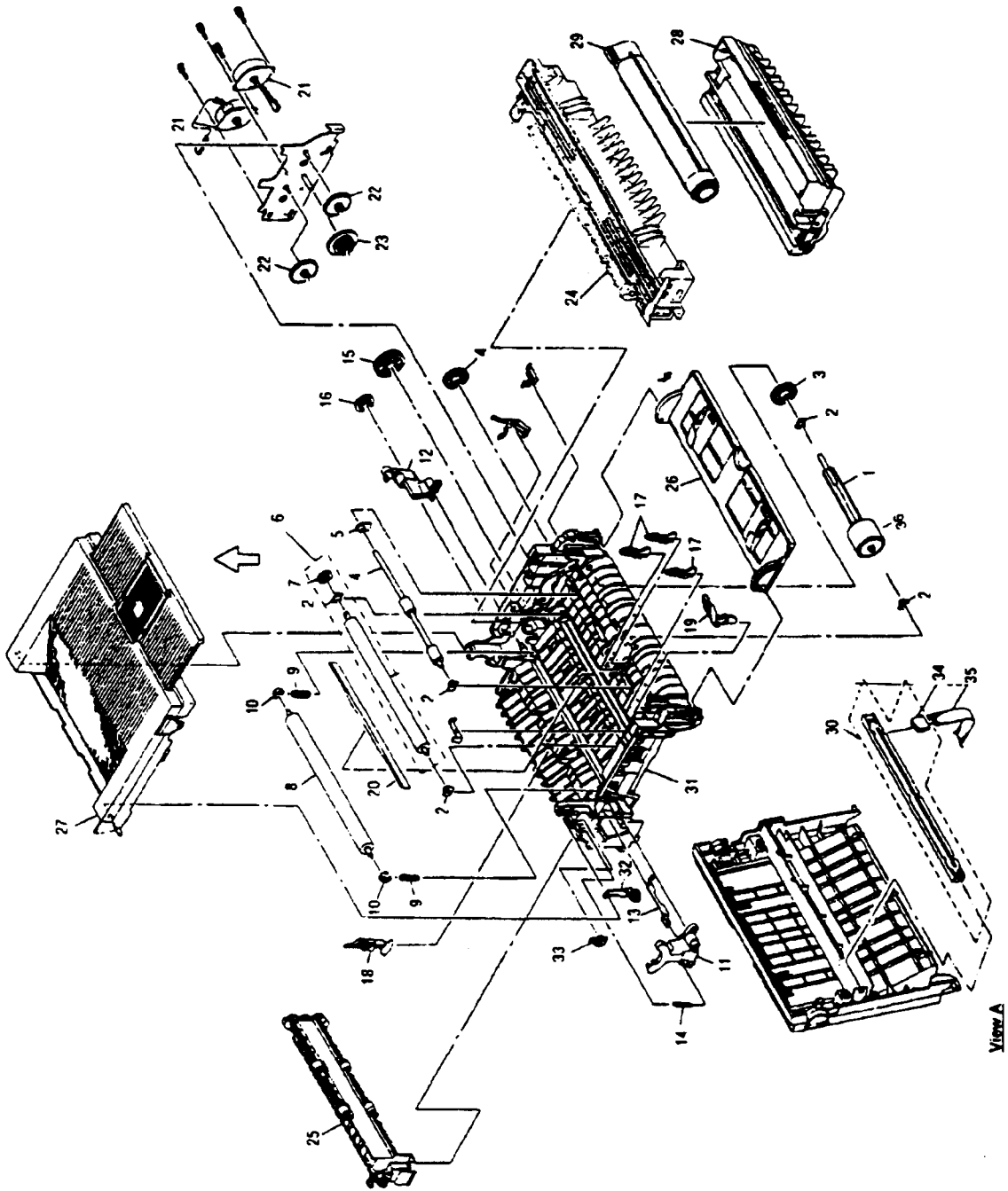
Figure 8-1 Lower Base Unit
