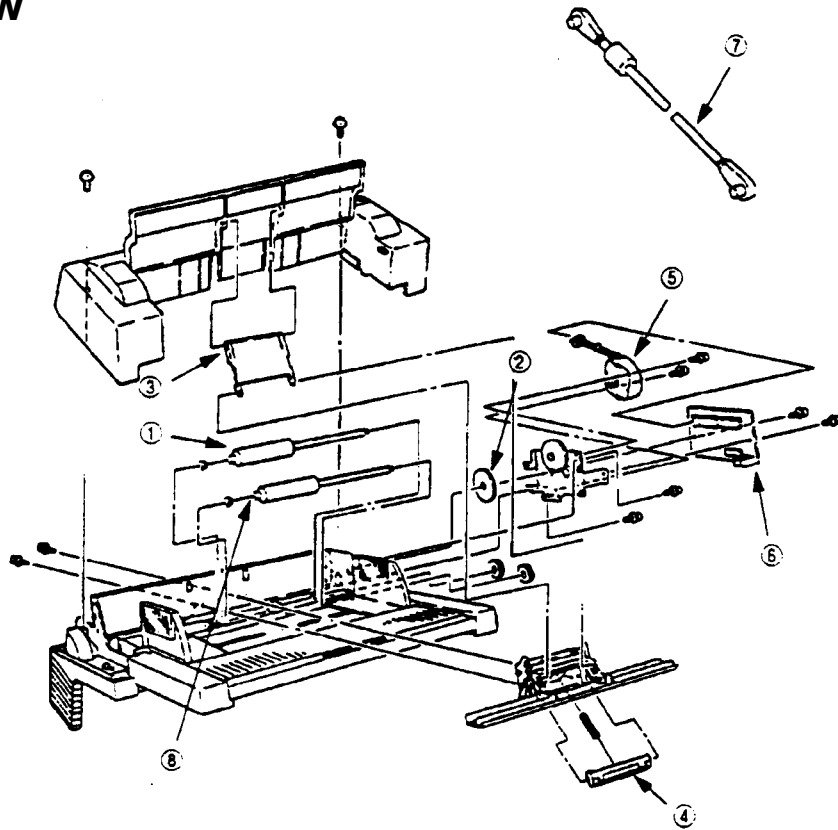
Fig. 6-1 Multi-Purpose Feeder
