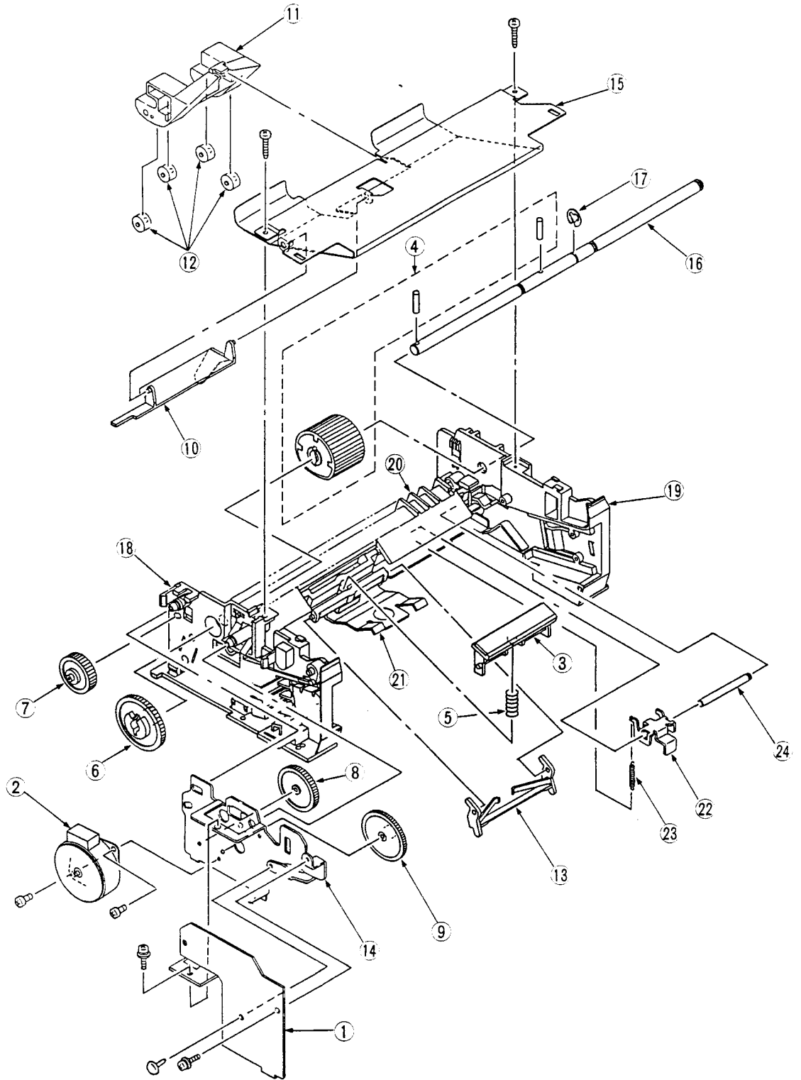
Figure 9-5 Paper Supply Unit
