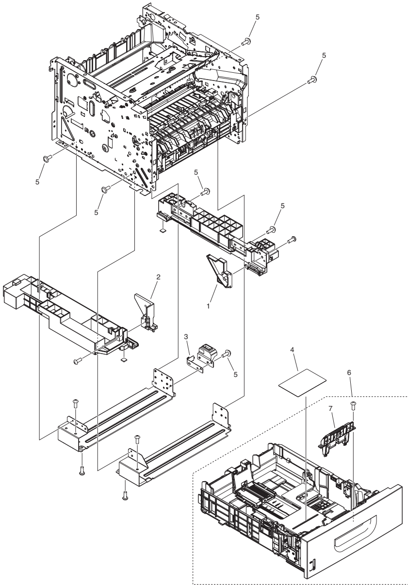
FIGURE 106A INTERNAL COMPONENTS 6 (EXCEPT MF5900 Series)
