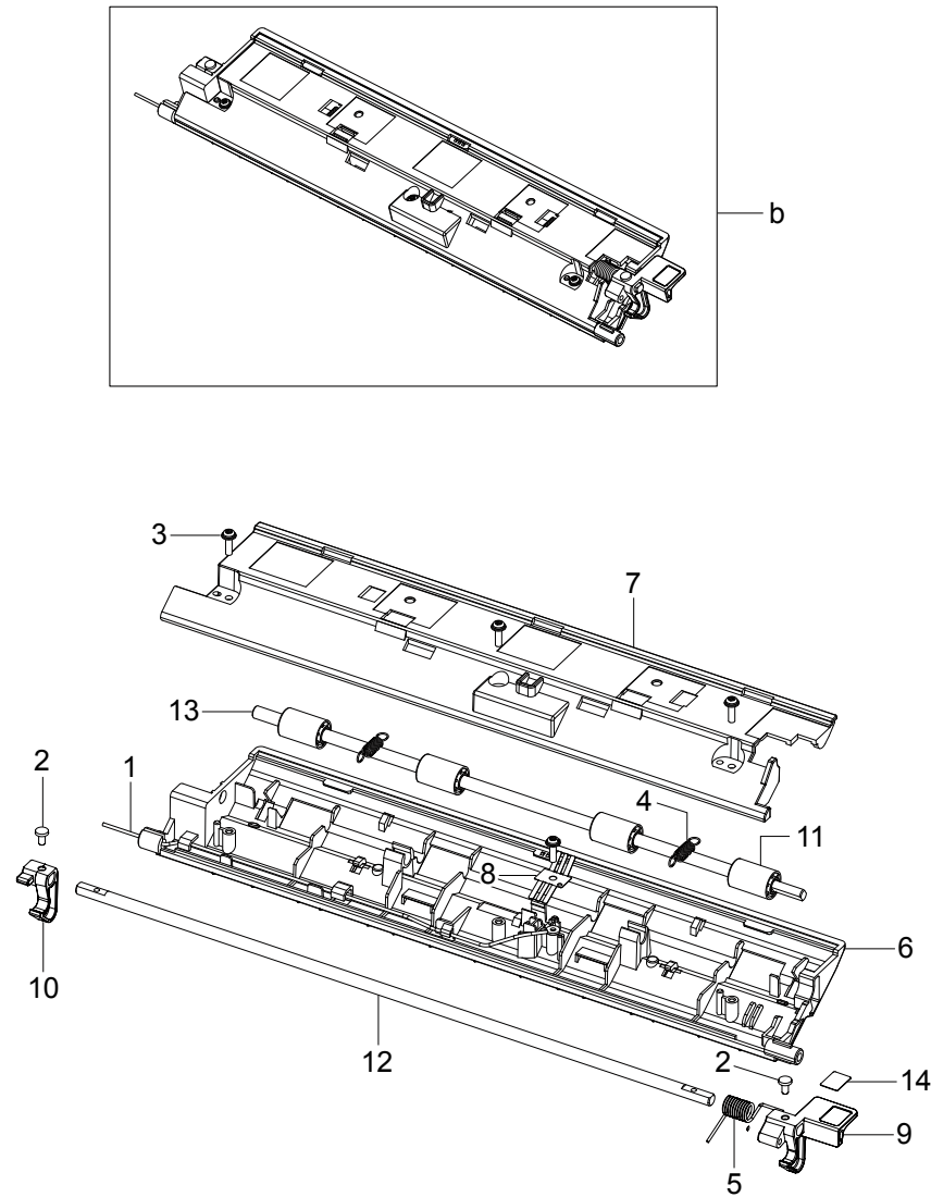
b. DADF GUIDE-FEED OUT
