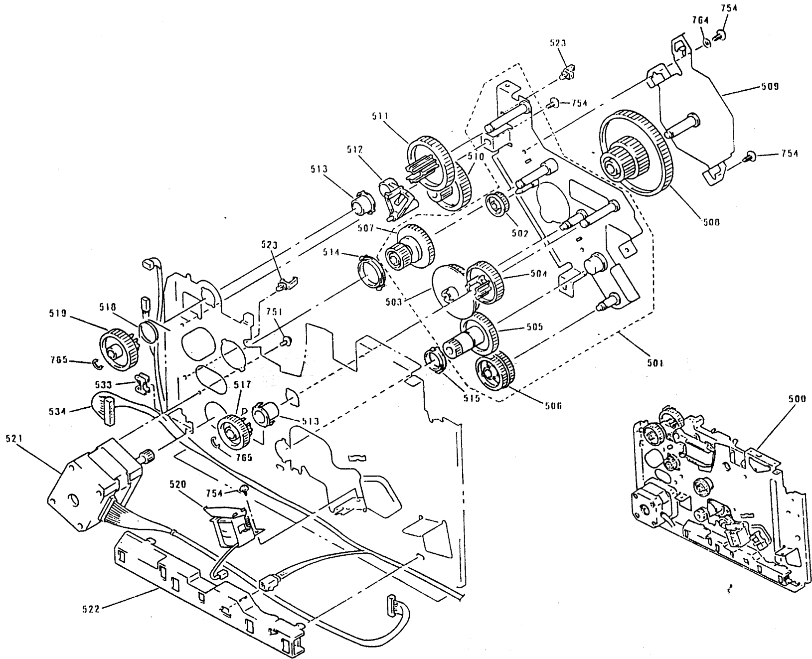
EXPLODED DIAGRAM FOR ACTION LASER 1600 / EPL-5600 (3)
