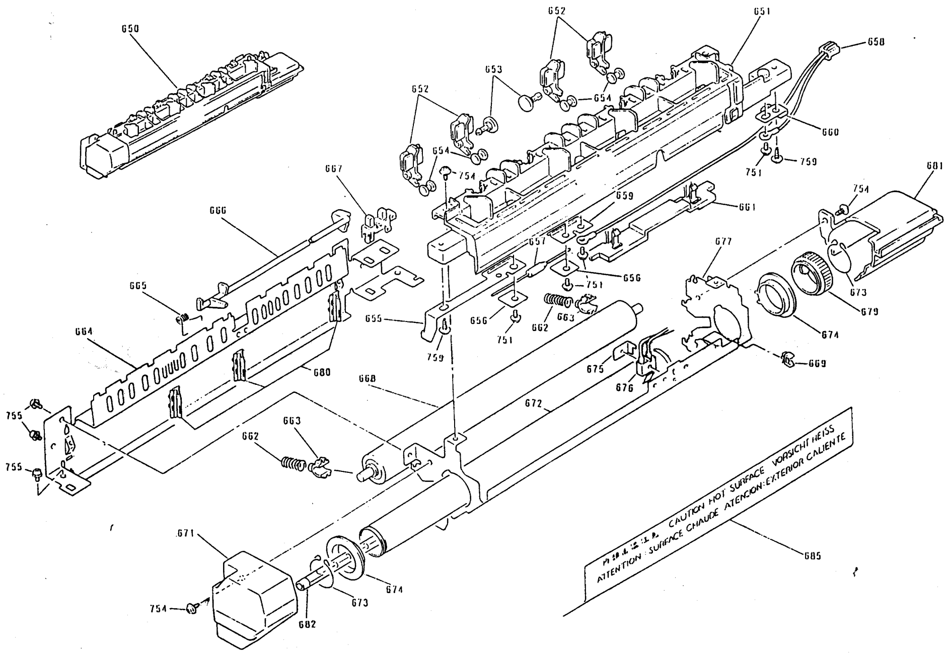
EXPLODED DIAGRAM FOR ACTION LASER 1600 / EPL-5600 (6)
