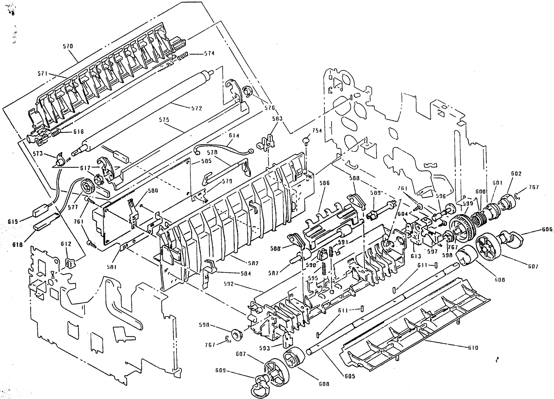
EXPLODED DIAGRAM FOR ACTION LASER 1600 / EPL-5600 (5)
