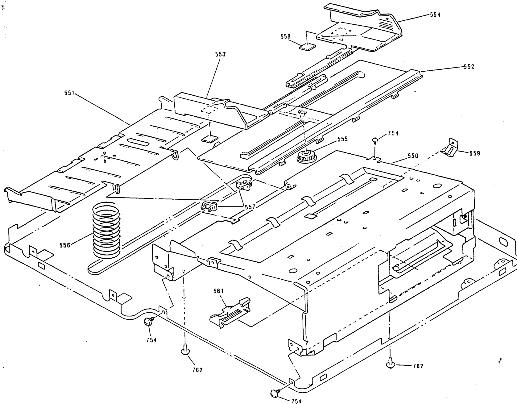
EXPLODED DIAGRAM FOR ACTION LASER 1600 / EPL-5600 (4)
