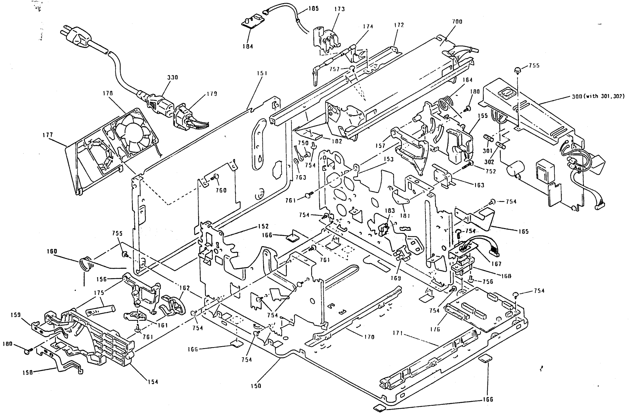
EXPLODED DIAGRAM FOR ACTION LASER 1600 / EPL-5600 (2)
