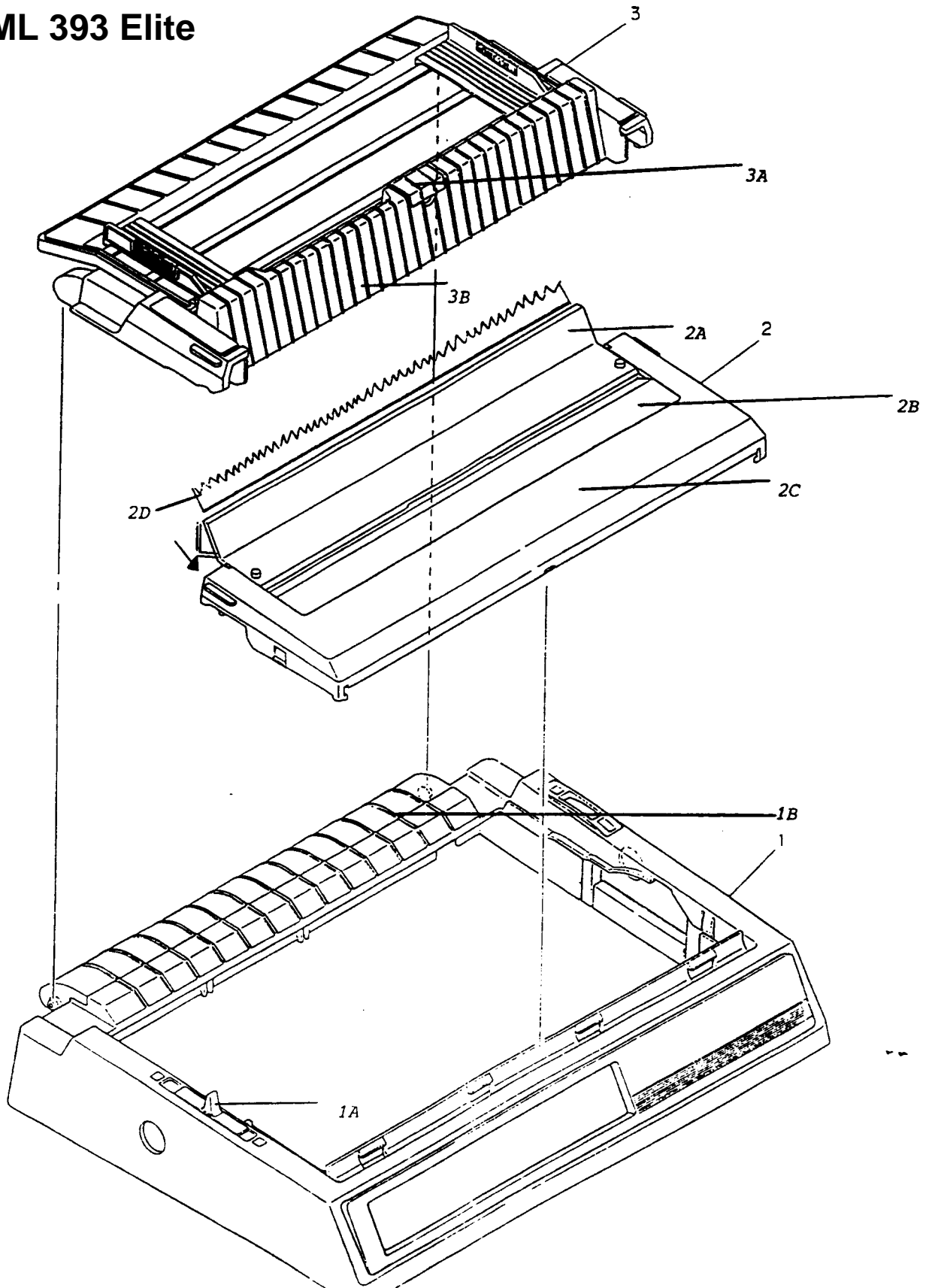
Upper Cover Assembly Monochrome Model
