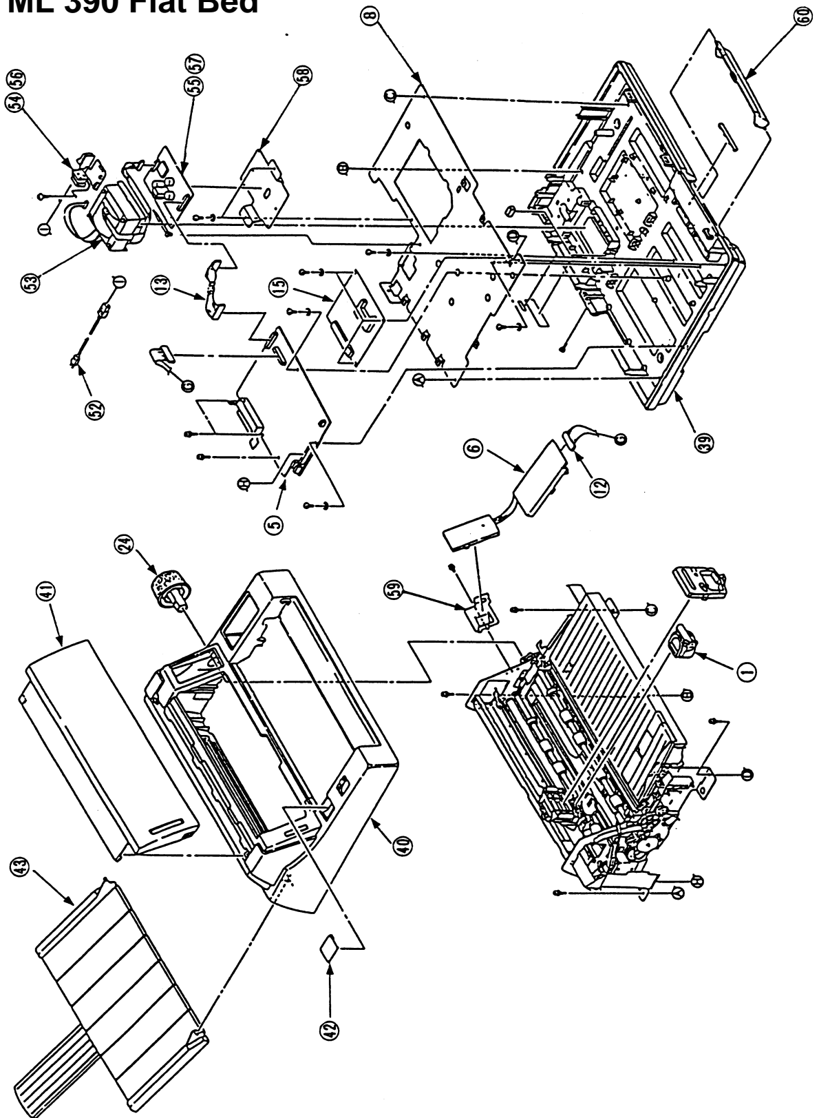
Printer unit (1/4)
