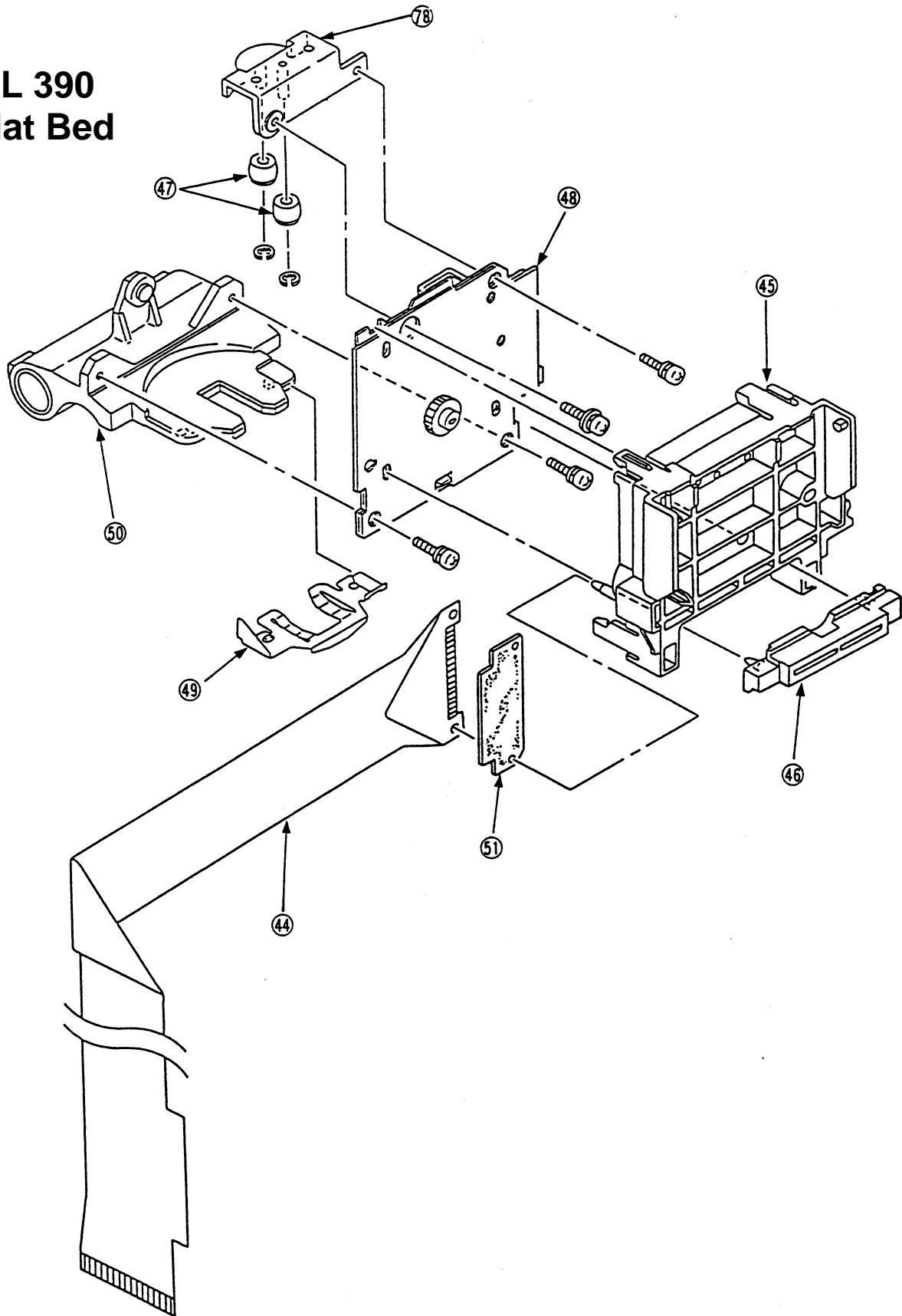
Printer unit (4/4)
