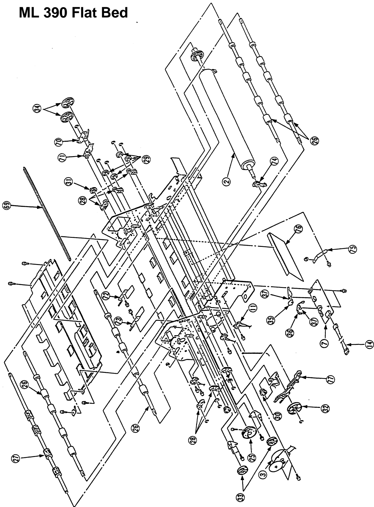
Printer unit (3/4)
