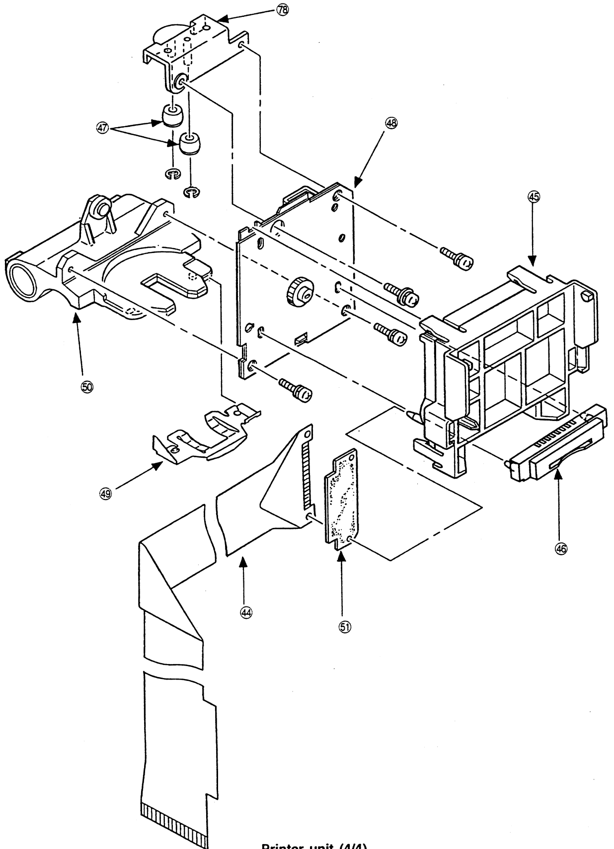
Printer unit (4/4)
