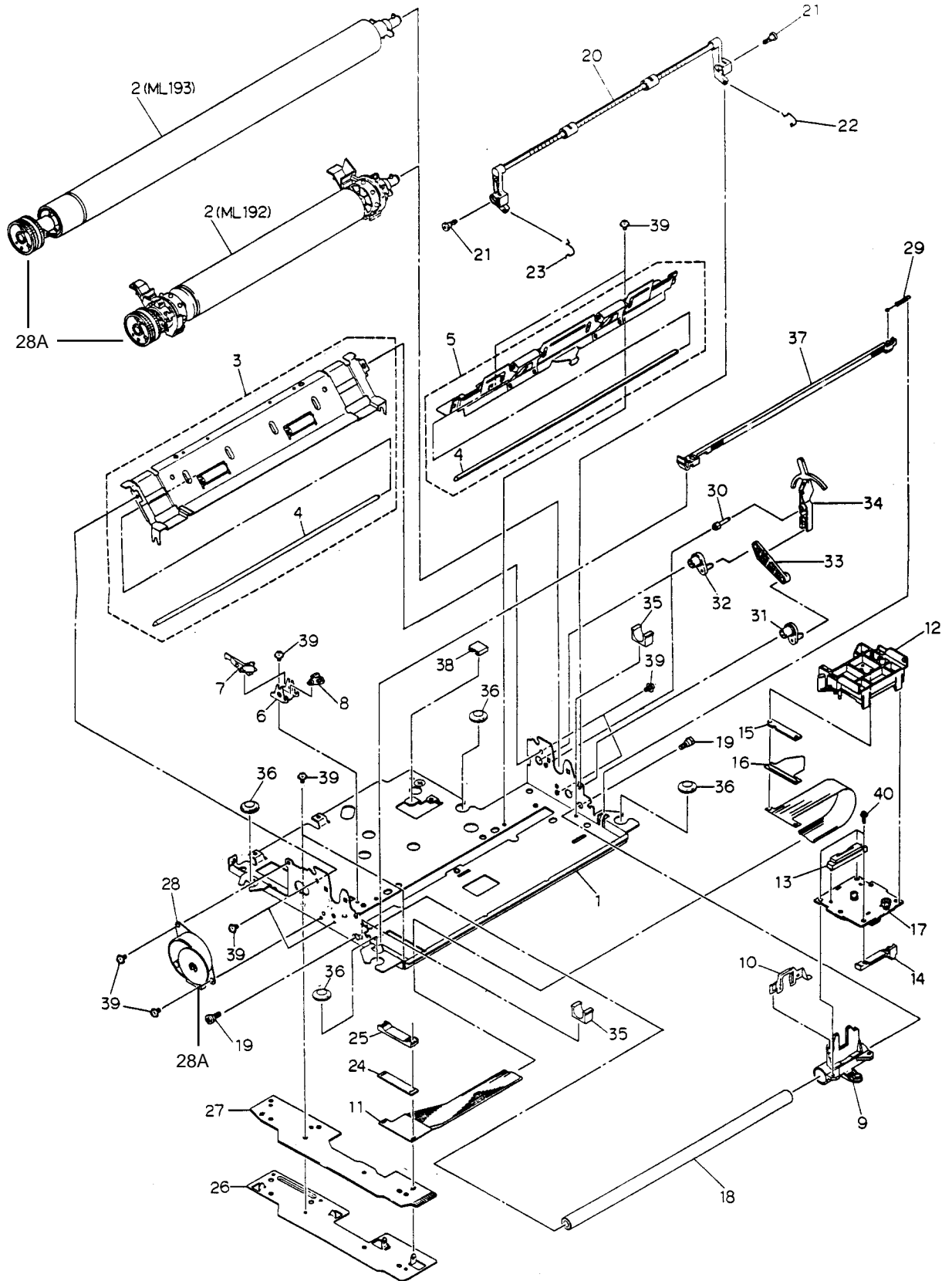
Figure 2 Printer Mechanism
