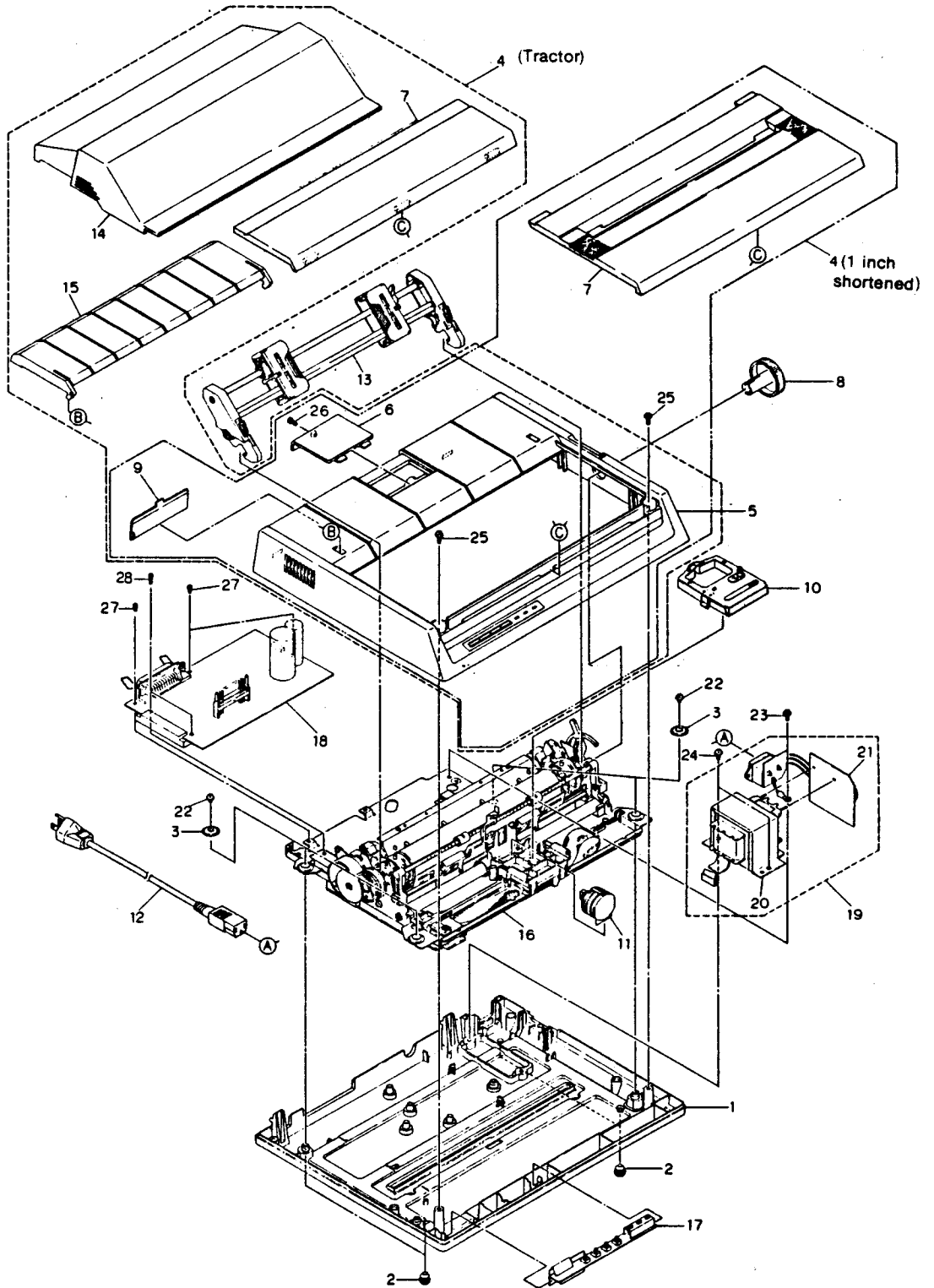
Figure 1 Printer Unit
